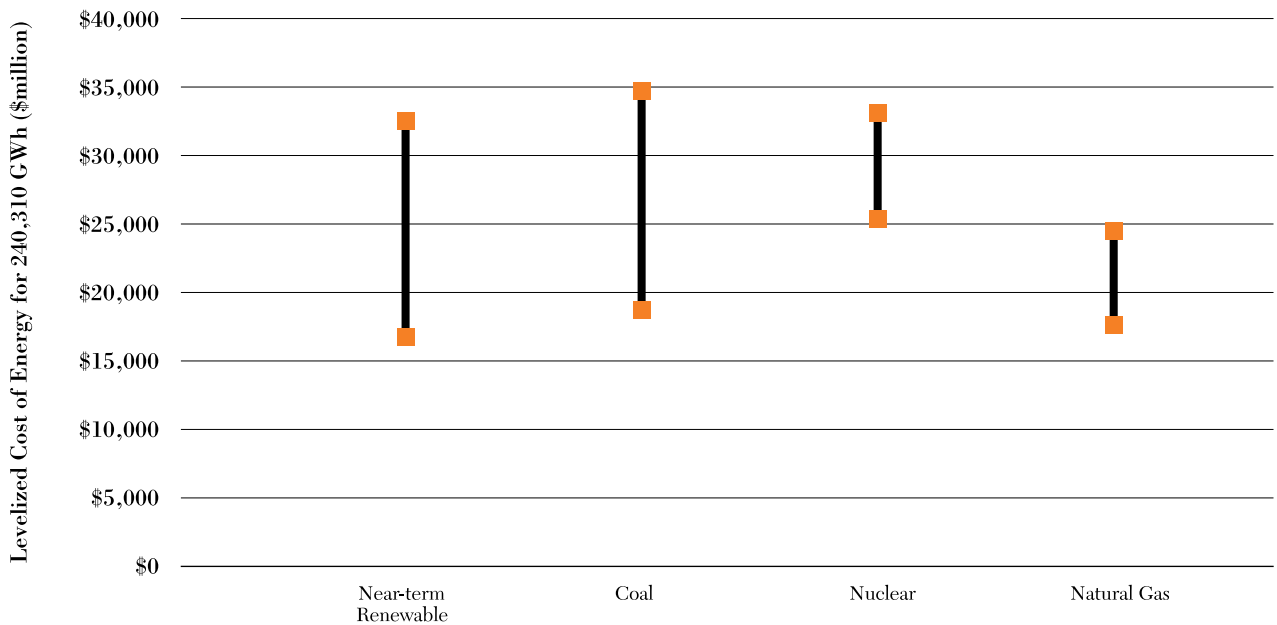
FIGURE 6 Illustrative Comparison of Costs for the Southeast’s Near-term Renewable Electricity Portfolio (approximately 240,000 GWh) with Equivalent Power Generation Using Conventional Electricity Resources
