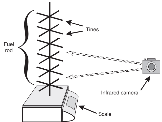
Fig. 2. The excelsior fuel rod experiments consisted of a scale supported upright steel fuel rod with perpendicular cross tines used to hold vertically arranged excelsior. The flame produced by burning excelsior is sampled with an infrared camera at 120 Hz.
