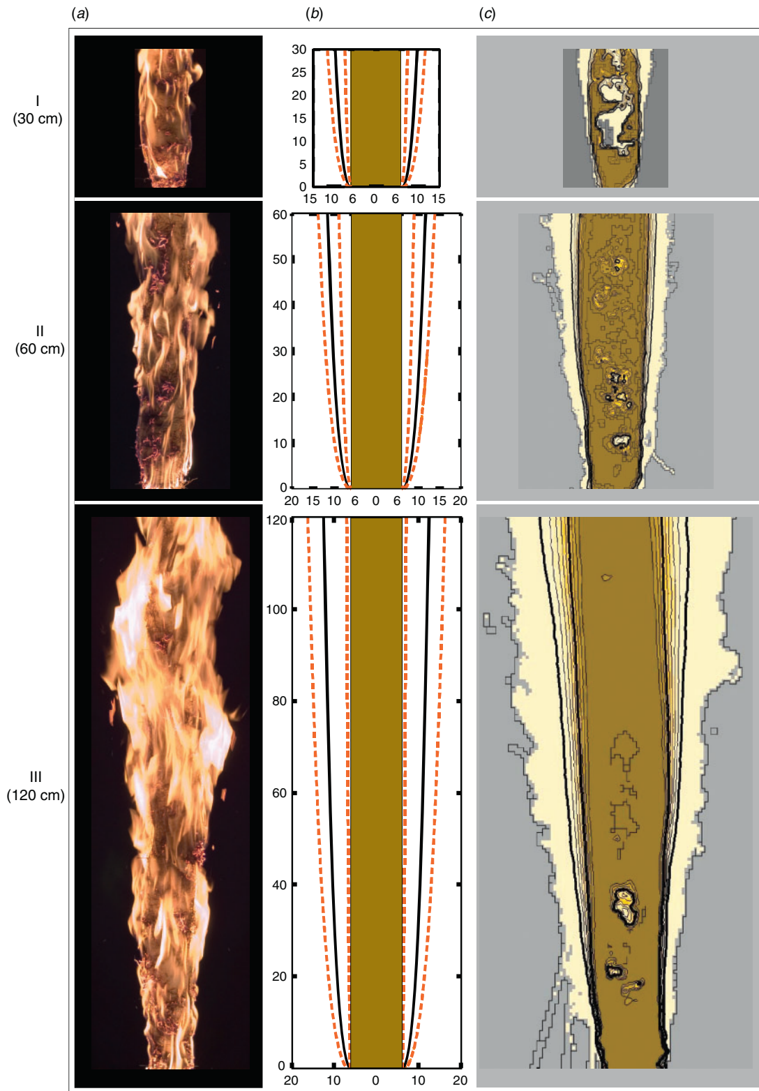
Fig. 4. Visible photographs of the 30, 60 and 120 cm tall excelsior fuel rods with an undulating flame edge indicating non-steady flame behaviour (a). Numerical solution for a 30, 60 and 120 cm-tall excelsior fuel rod having average mass loss rates of 5.92, 7.03 and 6.07 \text{g m}^{-1} \text{s}^{-1} respectively (b). The fuel is represented by the solid rectangle in the centre (spanning the horizontal distance -6.0 to 6.0 cm). The solid and dashed lines to either side of the fuel are the model results representing the mass-loss rate average (solid line) and \pm 2\sigma of that average (dashed lines). The frequency of flame presence is based on a radiant temperature threshold of 823 K (c). Contour lines are in 10% increments that outwardly decrease. The 50 and 10% presence contours are shown with heavier lines.
