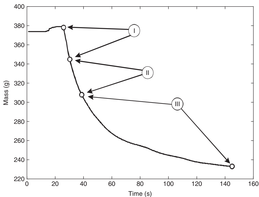
Fig. 3. Three main periods of burning can be identified in the mass loss data. Phase I is where ethyl alcohol is burned off. Phase II represents consistent external burning of the excelsior at a constant rate following complete combustion of the ethyl alcohol (constant slope). Phase III represents significant excelsior consumption where the excelsior fuel volume is decreasing and the interface between the excelsior and flame is no longer a vertical line.
