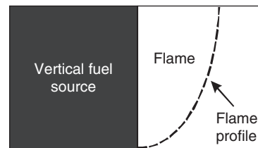
Fig. 1. A conceptual laminar flame profile developing from the surface of a cylindrical, vertical fuel source is shown. The combustion reaction occurs completely at the solid surface resulting in the combustion products forming the ‘flame’ profile.
