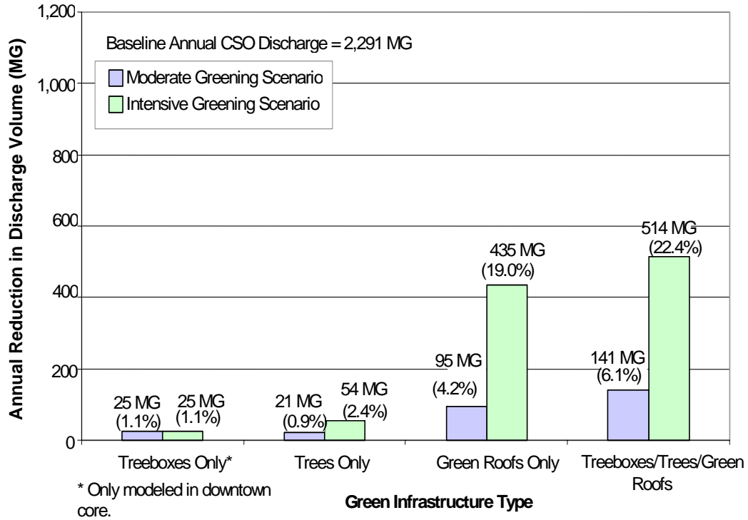
Figure 13: Reduction in CSO Discharge from the CSS
