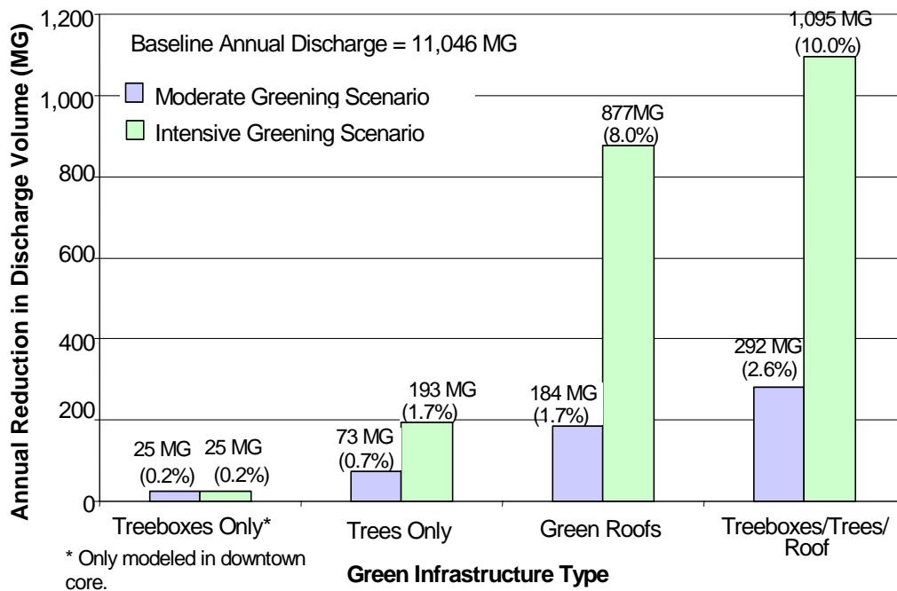
Figure 12: District-wide Reduction in CSO and Stormwater Discharge to All Waterbodies
