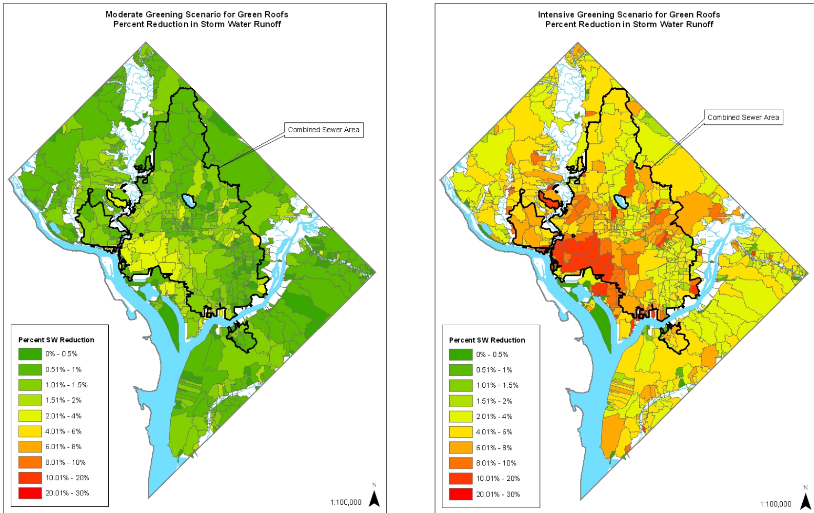
Figure A2: Sewershed comparison of Moderate Greening and Intensive Greening Scenarios for percent reductions in stormwater runoff from greenroof cover
