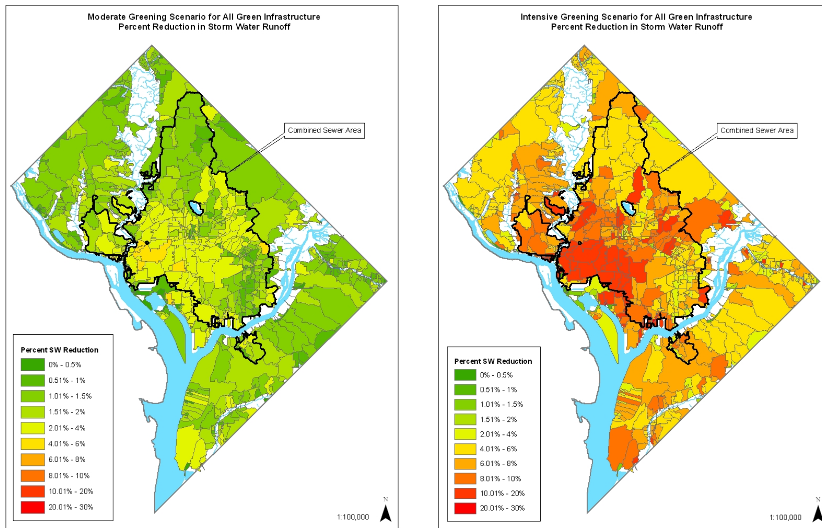
Figure 15: Sewershed comparison of Moderate Greening and Intensive Greening Scenarios for percent reductions in stormwater runoff for all green infrastructure (trees, greenroofs, and tree boxes)
