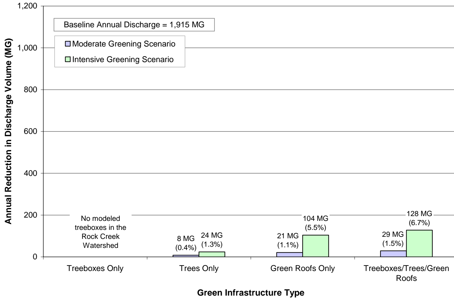
Figure A6: Reduction in CSO and Stormwater Discharge to Rock Creek
