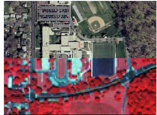
Figure C1: IKONOS Image
