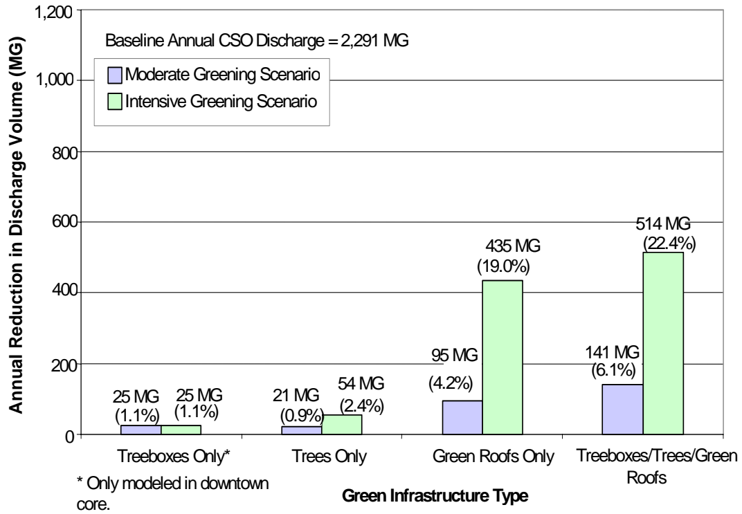
Figure 14: Reduction in Stormwater Discharge from the MS4 Area
