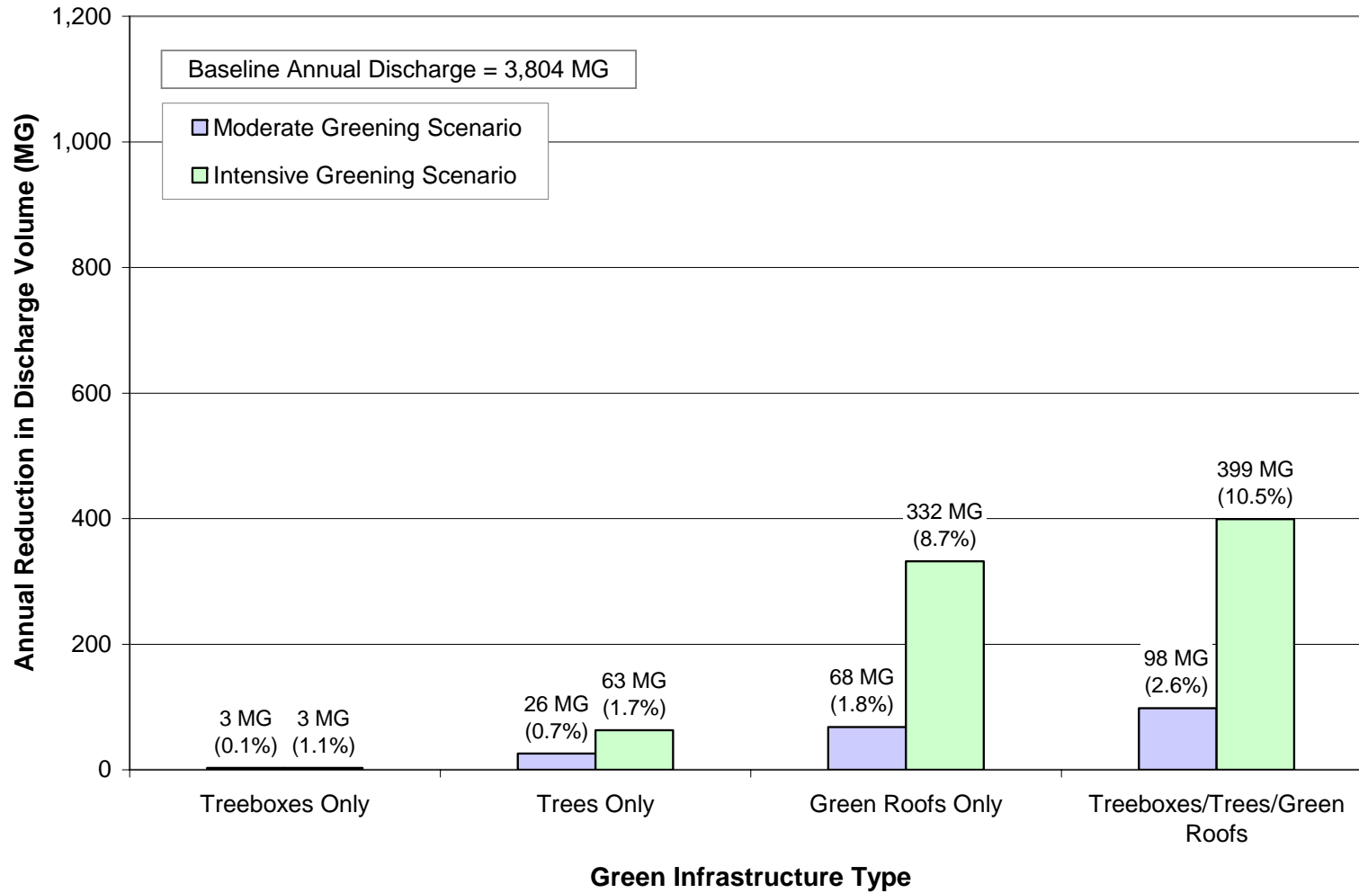
Figure A5: Reduction in CSO and Stormwater Discharge to the Potomac River
