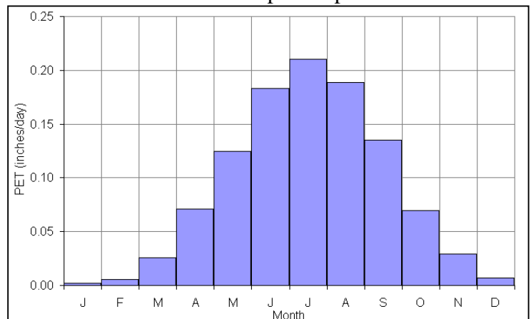
Figure B6: Evapotranspiration Rates for Washington, DC
