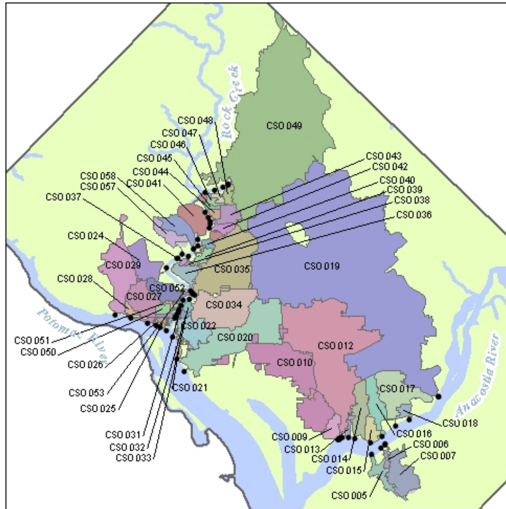
Figure A7: Map of CSS Sewersheds and Outfalls
