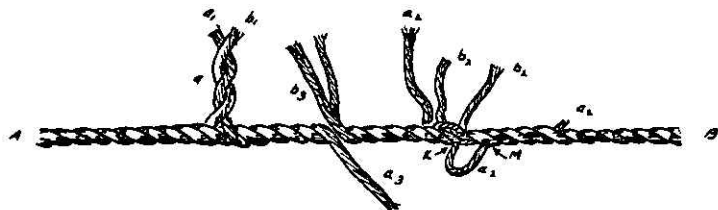
FIG. 22 LONG SPLICE (2)
