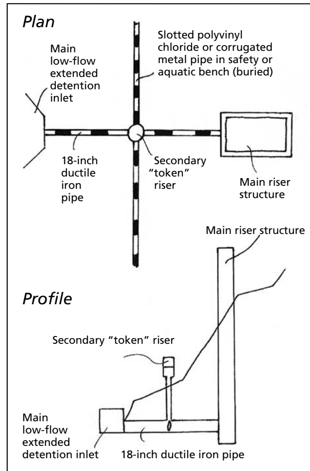
Figure 23. A secondary riser helps to keep permanent pools at safe elevations, even when outlets clog.
