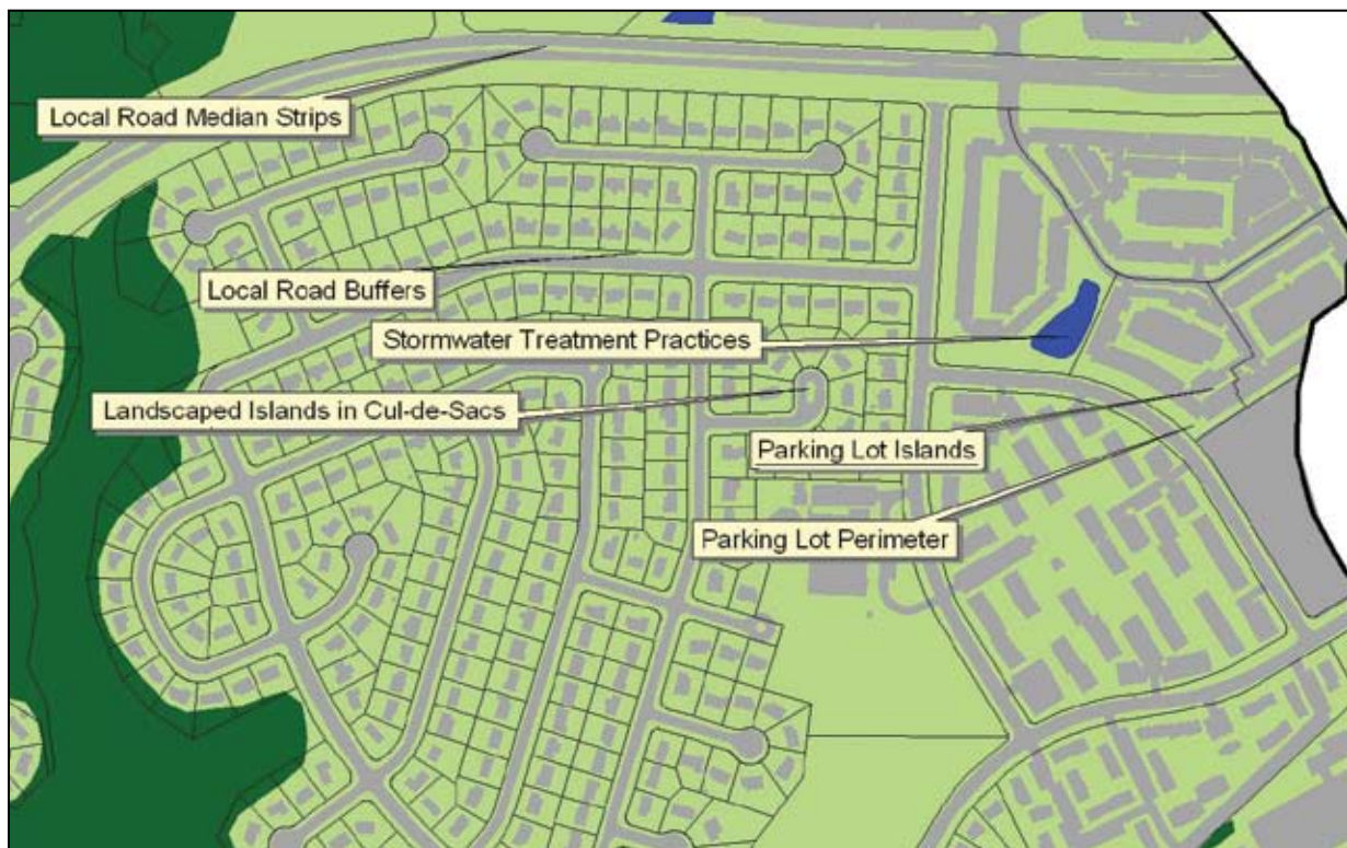
Figure 16. Development sites offer several potential planting areas.
