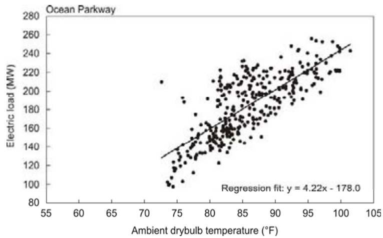
Figure 5-8. Electric load and temperature data for Ocean Parkway.
