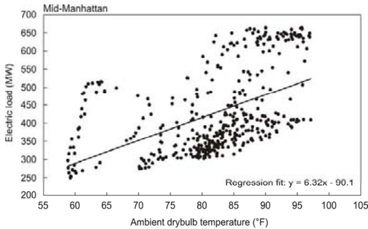
Figure 5-3. Electric load and temperature data for Mid-Manhattan West.
