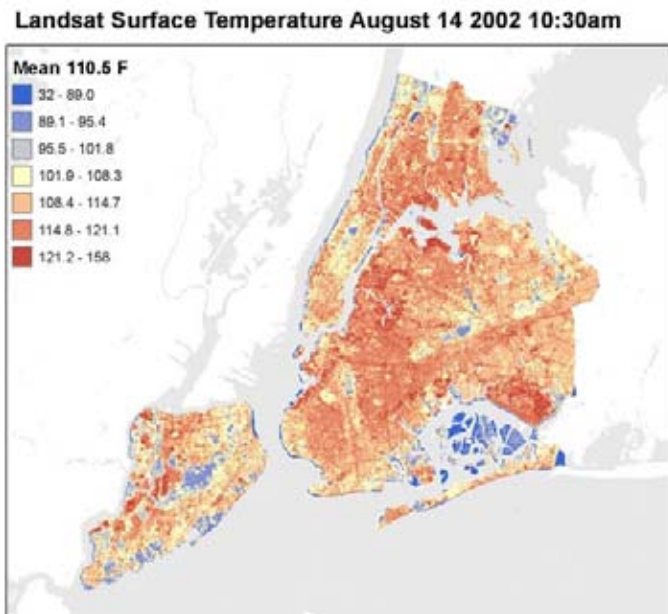
Figure 2-2. Remotely sensed thermal satellite data. Landsat ETM, August 14, 2002 at 10:30 AM, Band 6, resolution is 60 meters.
