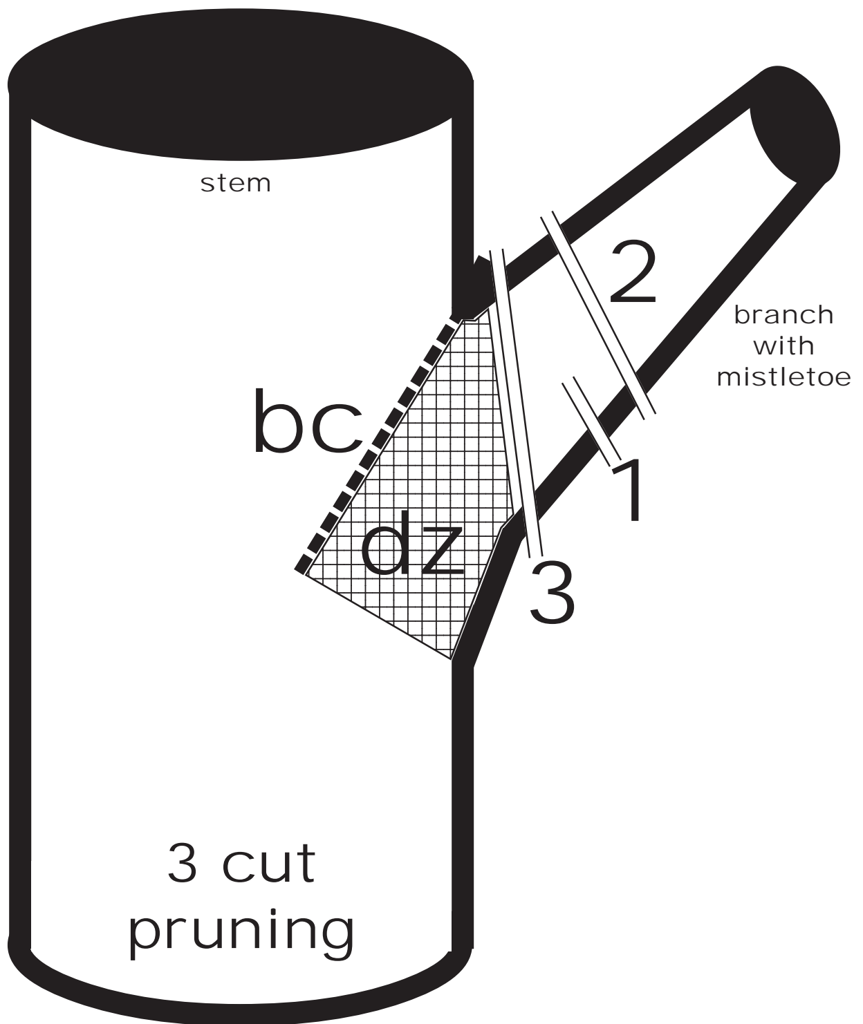
Figure 12: Diagram of stem - branch confluence area with a three-cut pruning prescription applied (in cut order) for a mistletoe infected branch where the infection is greater than 14 inches away along the branch. Defensive zone = dz. Bark chine = bc.
