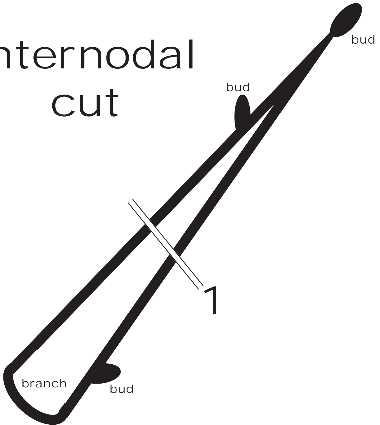
Figure 11: Diagram of an abusive, improper, and damaging internode cut. Other terms used for this abusive cut include topping, tipping, hedging, hat-racking, and trimming. It is not the size of tree part cut (stem, branch, or twig) but the internodal location which makes this cut improper and damaging.
