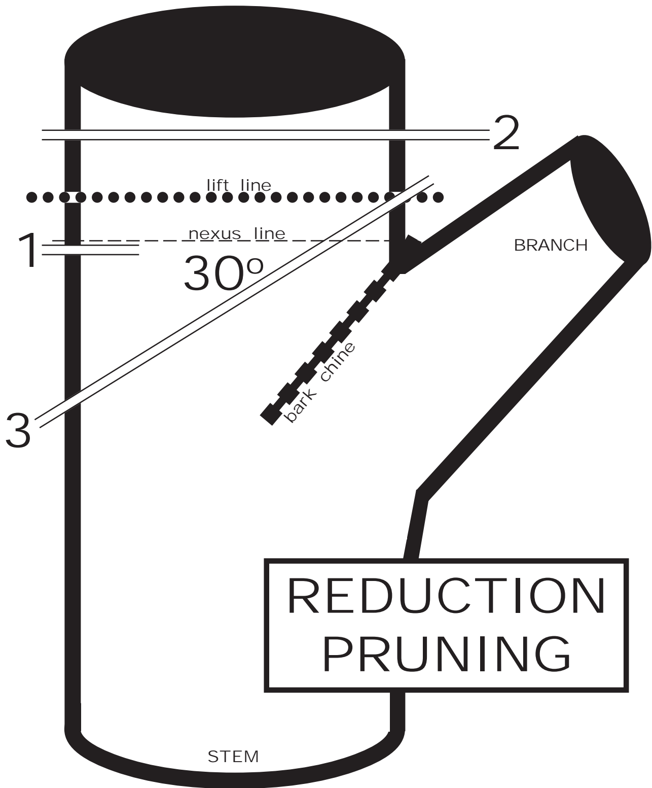
Figure 13: Diagram of stem - branch confluence with reduction cut lines, in numbered order greater than 14 inches below a stem mistletoe infection. Note the final (3 rd ) cut is at 30° down angle from the branch side of the lift line. The lift line is 1/9 of the stem diameter, or at least 3X saw kerf thickness above the nexus line.
