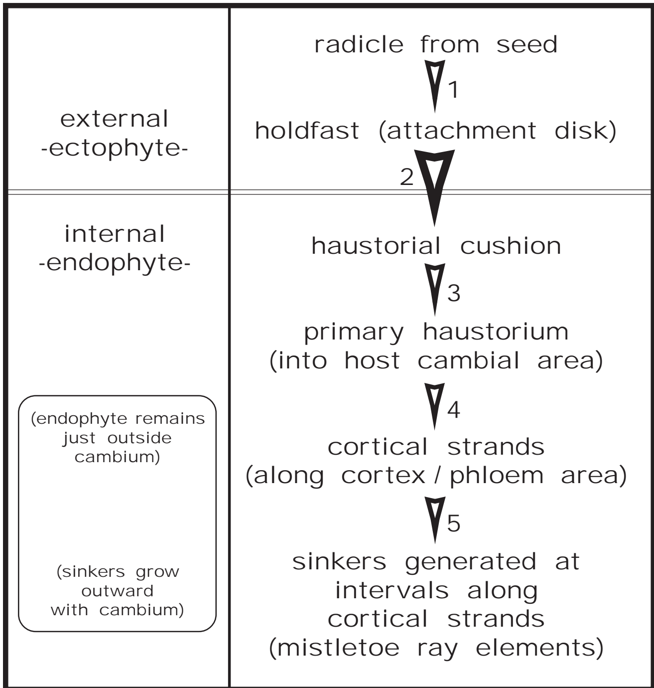
Figure 5: Mistletoe infection process steps. The primary haustoria establishes initial contact with host phloem, cambium area and xylem. Cortical strands establish indirect contacts with host phloem. Sinkers establish direct (5%) and indirect (95%) contacts with host xylem.
