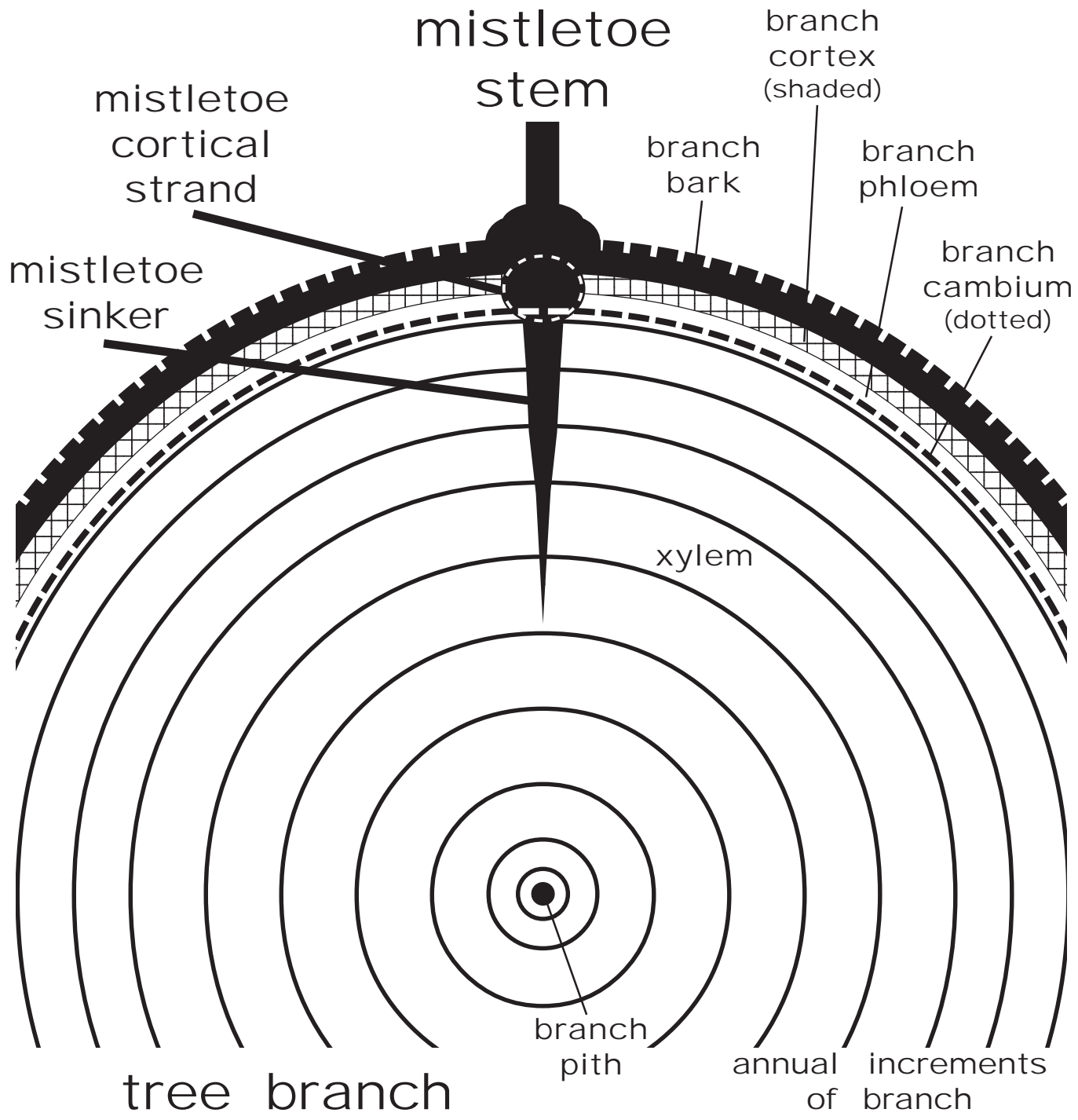
Figure 6: Simplified diagram of a tree branch cross-section with a mistletoe infection. Shown is a cortical strand and associated sinker (mistletoe ray element). The sinker is maintained with strand cambium aligned with the branch cambium.
