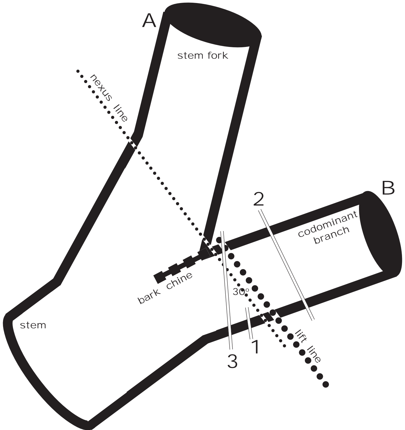
Figure 15: Diagram of a 3 cut reduction (in numbered order) of codominant branch / fork (B) greater than 14 inches below a mistletoe infection. Note the final (3 rd ) cut is at a 30° down angle from the branch side of the lift line. The lift line is 1/9 of the stem diameter, or at least 3X saw kerf thickness, above the nexus line.
