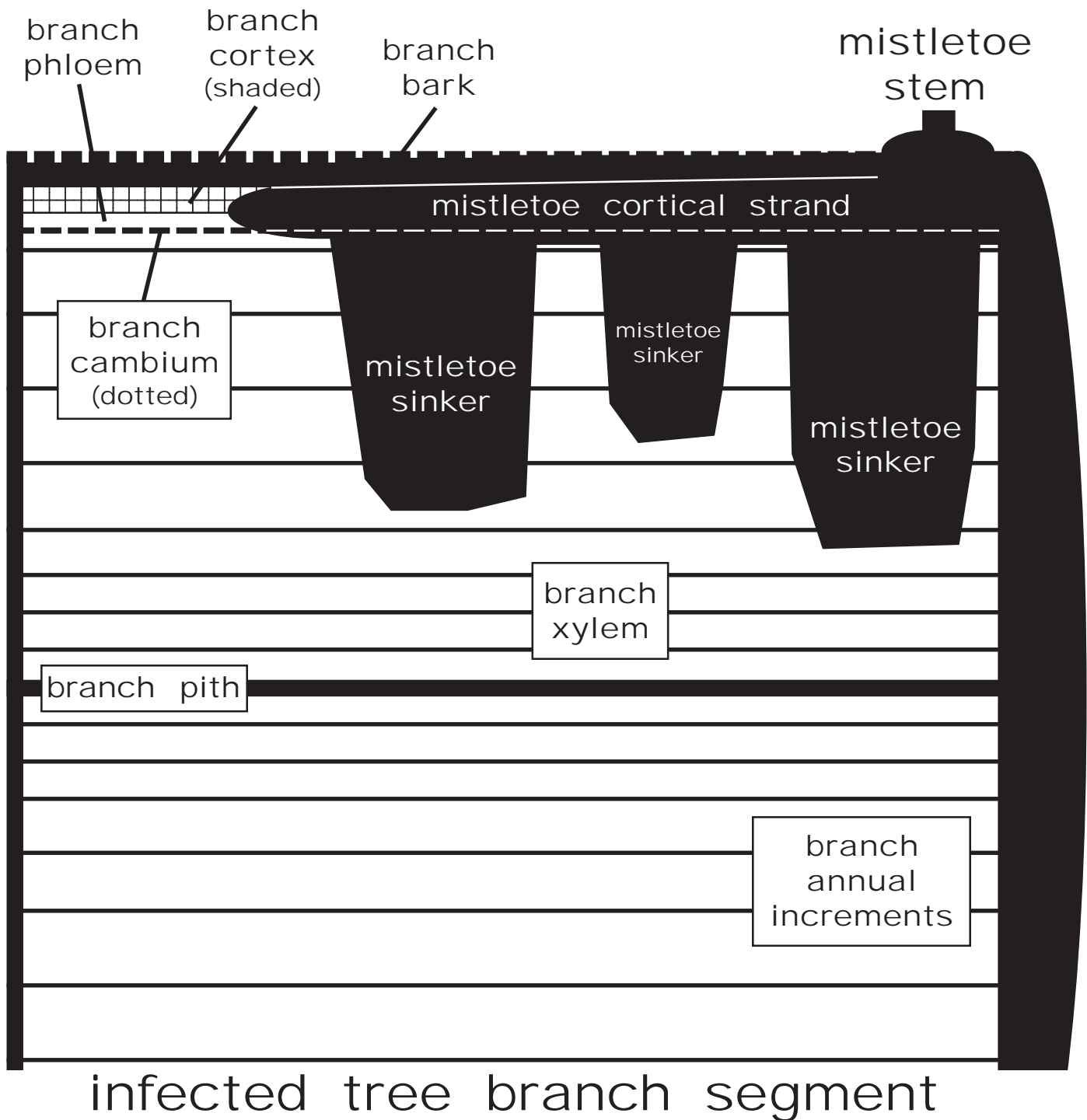
Figure 7: Simplified diagram along the longitudinal central axis of a branch with a mistletoe infection. Shown is a cortical strand and associated sinkers (mistletoe ray elements). The sinkers are maintained and grow outward with strand cambium aligned with the branch cambium.
