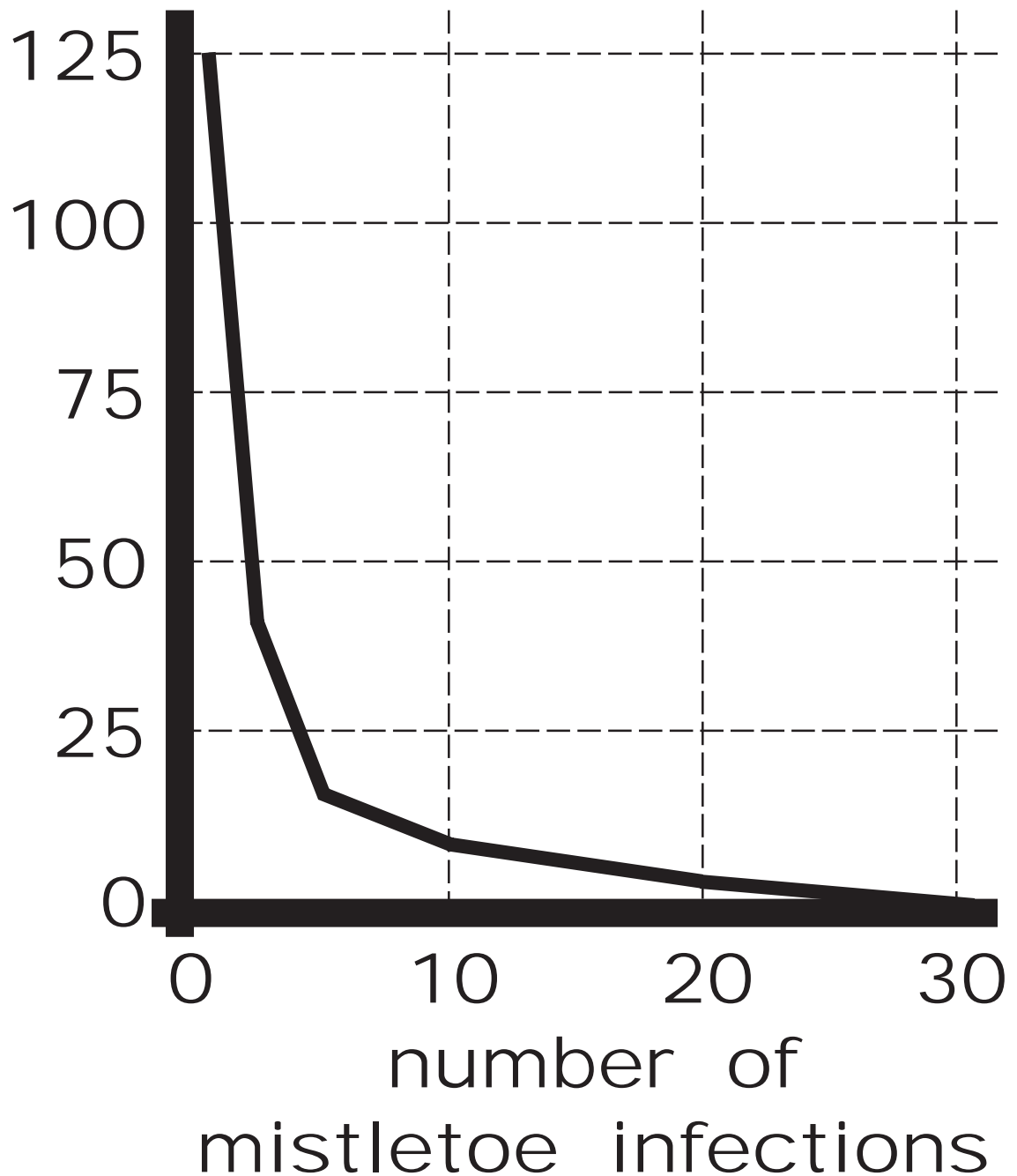
Figure 10: Representative example of the number of individual mistletoe infections (plants) per sampled tree. Percent of all trees with infections is 28%. (after Aukema & del Rio, 2002)
