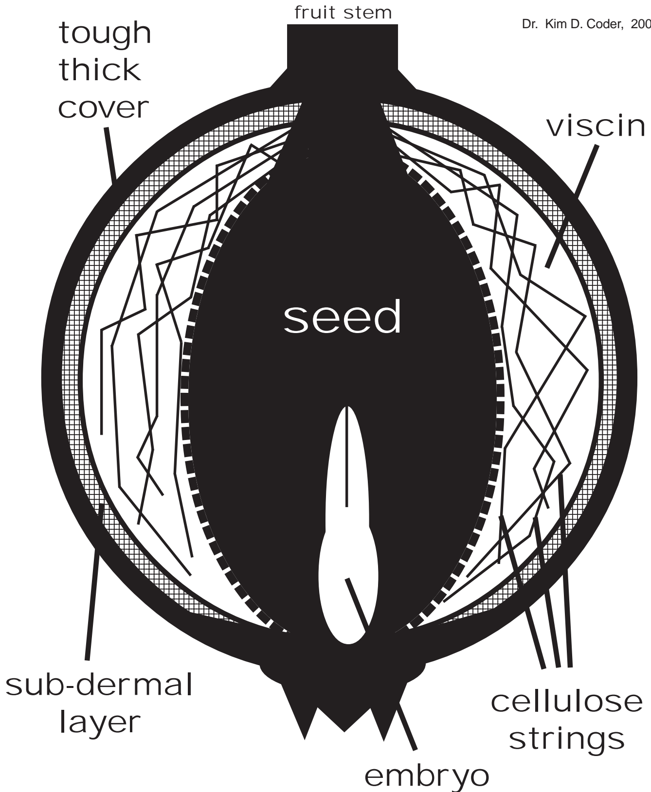
Figure 3: Simplified diagram of mistletoe fruit in cross-section. The fruit cover minimizes oxygen reaching the seed and moisture loss. The viscin is a pectin jelly which, when exposed to air, will dry and glue the seed to a twig. The cellulose strings will tangle with, and spread out over, a bark surface maximizing surface area contact for seed attachment.
