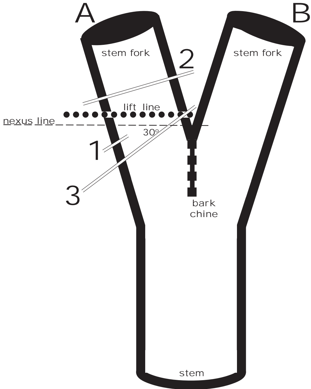
Figure 14: Diagram of forked stem with 3 cut lines in numbered order for reduction pruning stem fork A (left fork) greater than 14 inches below a stem fork mistletoe infection. Note the final (3 rd ) cut is at a 30° down angle from the branch side of the lift line. The lift line is 1/9 of the stem diameter, or at least 3X saw kerf thickness, above the nexus line.
