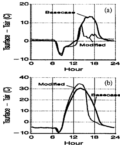
Fig. 6. Difference between measured surface temperatures and outdoor air temperature for days before and after the placement of shade trees (September 1) at Site T1, (a) wall; (b) roof. Solid line represents the average for 7 clear days between August 17 and August 31, when the surfaces were not shaded. Dotted line represents average for 10 clear days between September 1 and September 15, when the surfaces were shaded. The shaded wall is cooled beginning around 2 p.m., by as much as 12°C. In the presence of shade trees, the roof is slightly warmer in the morning and early afternoon. Beginning around 3:30 p.m., the surface is shaded and cooled as much as 20°C.
